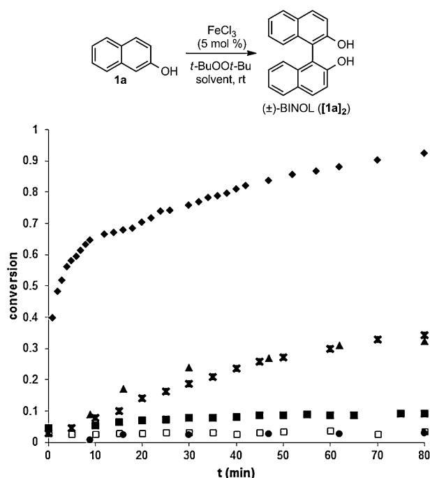
Figure 1. Effect of the solvent on the oxidative coupling of 2-naphthol ( 1a ). [a] Conditions: 1a (1 mmol), FeCl 3 (0.05 mmol), t BuOO t Bu (2.5 mmol), solvent (1 M), room temperature. The following solvents were used: (♦) 1,1,1,3,3,3-hexafluoropropan-2-ol (HFIP); (▲) 2,2,2-trifluoroethanol (TFE); (*) 2,2,2-trichloroethanol; (■) 1-phenyl-2,2,2-trifluoroethanol; (□) 1,1,1-trifluoropropan-2-ol; (●) 1,2-dichloroethane. The reaction progress was monitored by HPLC.
